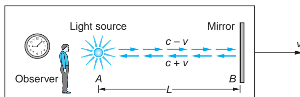
FIGURE 1-5 Light source, mirror, and observer are moving with speed v relative to the ether.
